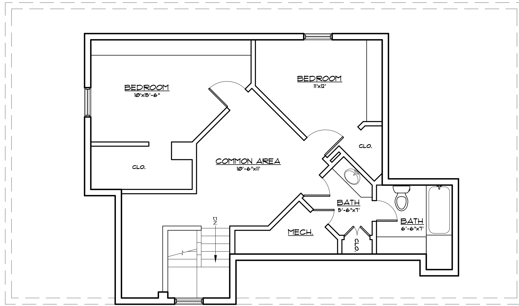
3RD FLOOR SCALE: 3/16" = 1'-0"
