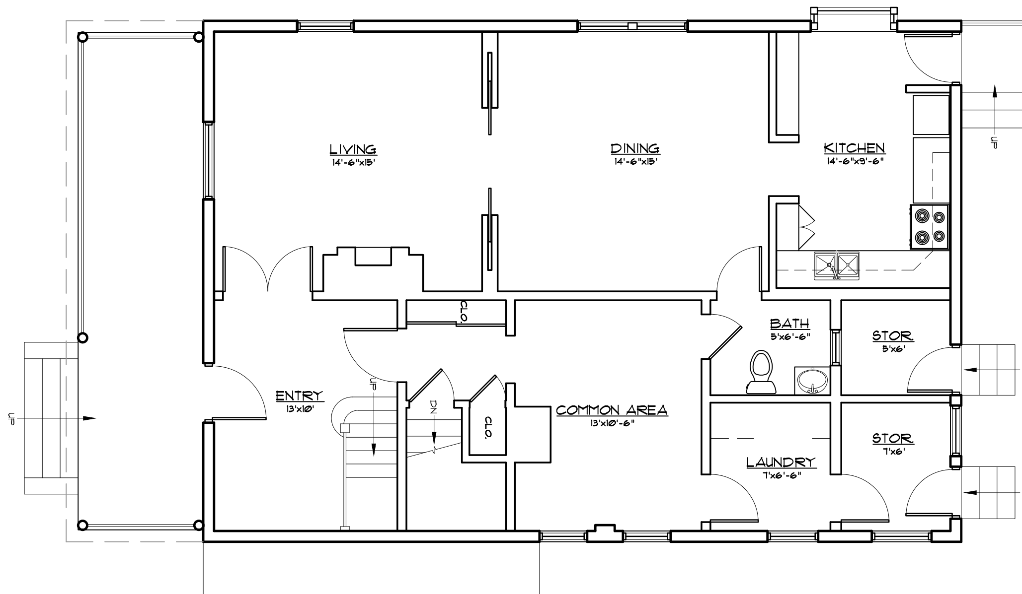
1ST FLOOR SCALE: 3/16" = 1'-0"
